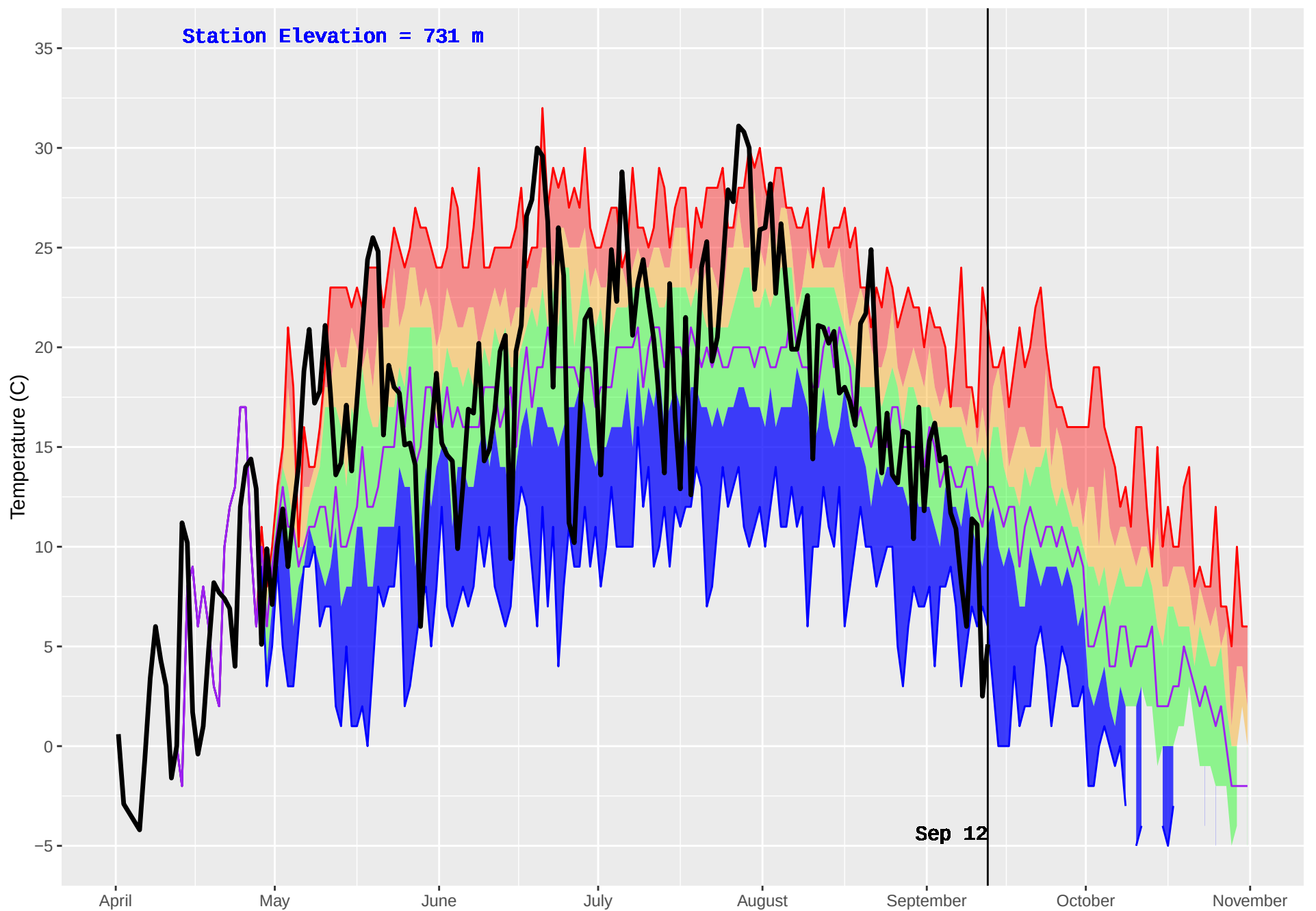
FIRESIDE (440) : Historical (1996–2016) and Current (2018) Daily Temperature
