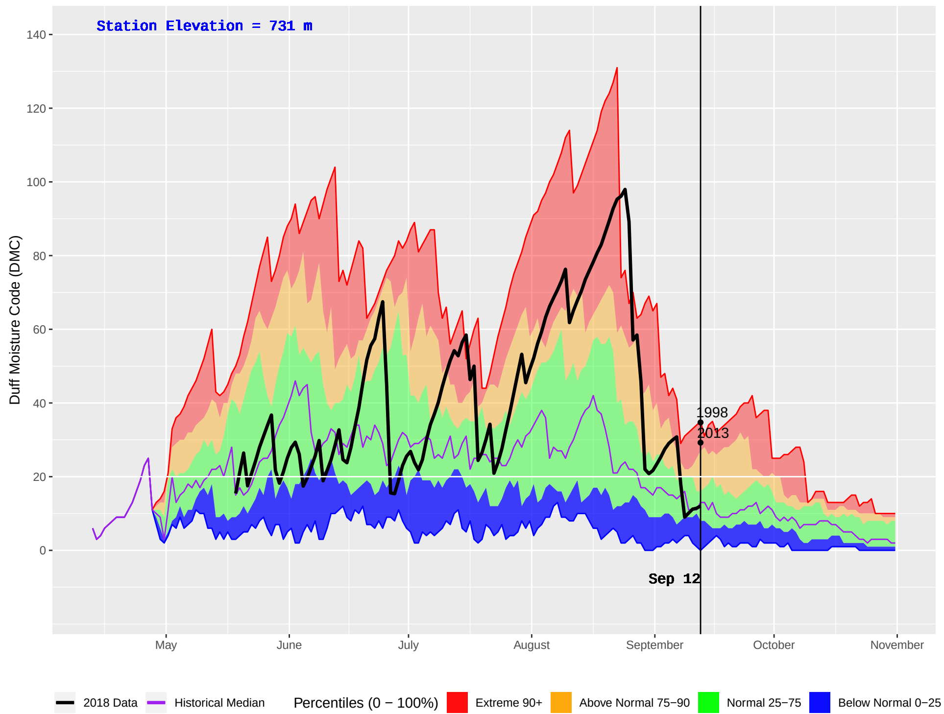
FIRESIDE (440) : Historical (1996–2016) and Current (2018) Daily Duff Moisture Code (DMC)
